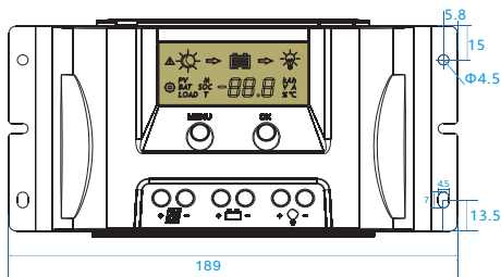
MT1050/1550-EU
