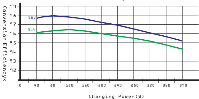
12V Conversion Efficiency Curves Solar Module MPP Voltage 18V/36V
